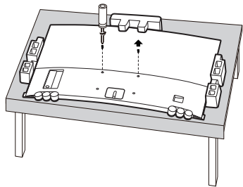
1 从后壳上取下挂架螺钉
